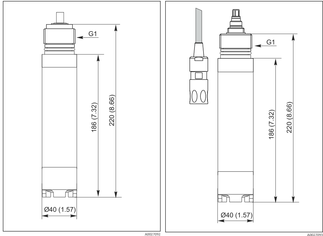
14 Version with fixed cable
