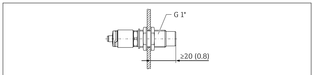
4 Bore hole in silo wall with lock nuts, can be ordered as an accessory → 19
