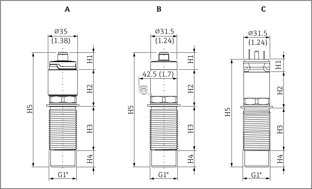
9 Dimensions of Nivector. Unit of measurement mm (in) A Nivector FTI26 plastic with M12 plug B Nivector FTI26 stainless steel with M12 plug (with ground terminal for hazardous area) C Nivector FTI26 stainless steel with valve plug
