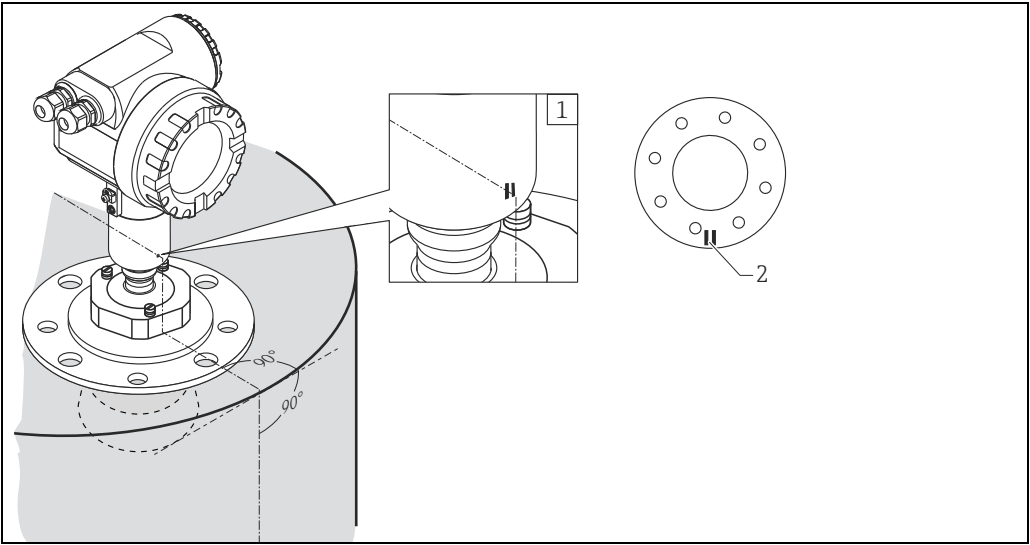
1 Marking on sensor 2 Marking on flange
