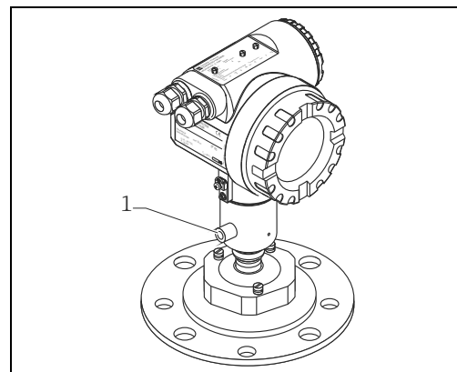
1 Purge air connection G 1/4" (max. torque 3.5 Nm (2.581 lbf ft))
