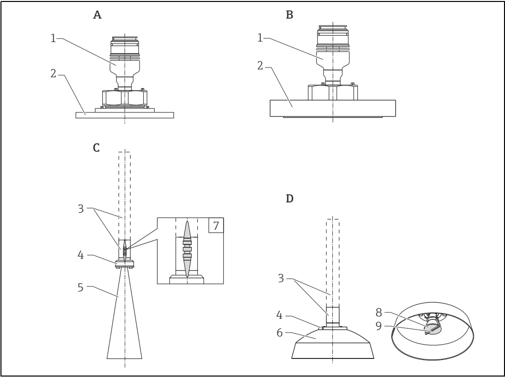
A Alignment device with Endress+Hauser UNI flange B Alignment device with standard flanges C Horn antenna (with antenna extension) D Parabolic antenna (with antenna extension)
