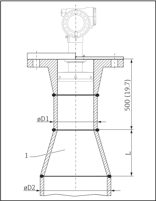
Recommended increase in diameter for retrofit of mechanical systems
