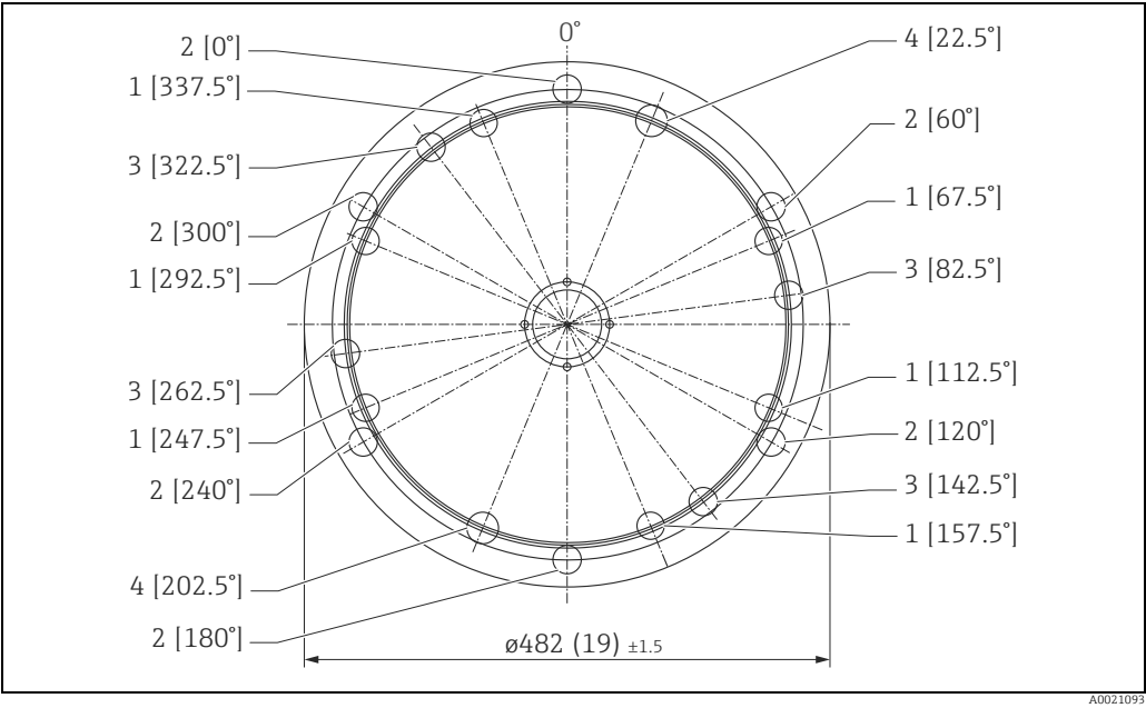
Endress+Hauser UNI flange. Engineering unit mm (in).
