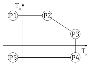
25 316L housing; process temperature -40 to +130 °C ( -40 to +266 °F)
