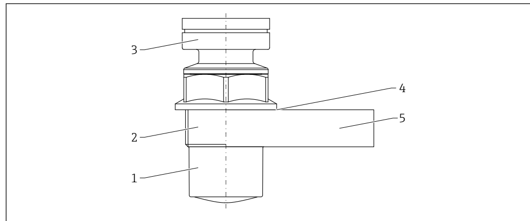
44 Material; encapsulated PVDF antenna, 40 mm (1.5 in)
