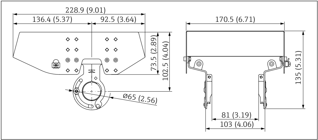
48 Dimensions of weather protection cover, 316 L, XW112. Unit of measurement mm (in)
