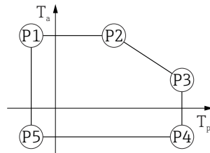
24 316L housing; process temperature -40 to +80 °C ( -40 to +176 °F)
