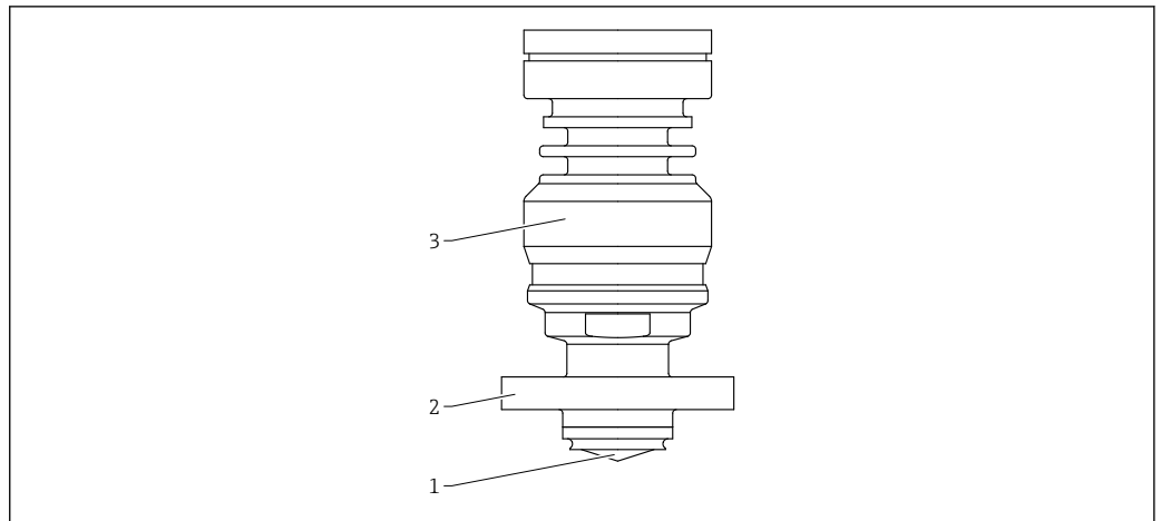
Antenna cladded flush mount, PEEK, 20 mm (0.75 in), NEUMO BioControl D25
