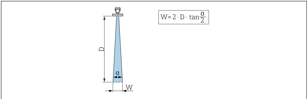
18 Relationship between beam angle α, distance D and beamwidth diameter W
