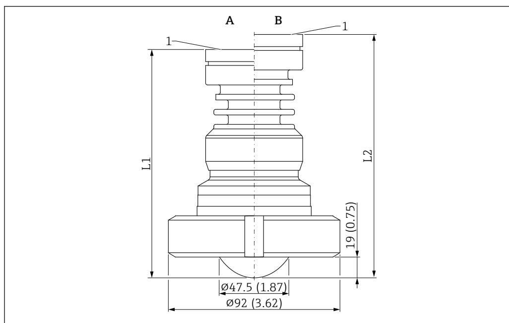
56 Dimensions of antenna, cladded flush mount, PTFE, 50 mm (2 in), slotted nut DIN11851. Unit of measurement mm (in)
