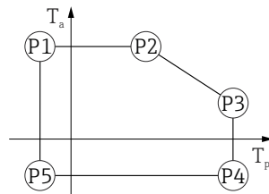
36 316L housing, hygiene; process temperature -40 to +80 °C ( -40 to +176 °F)
