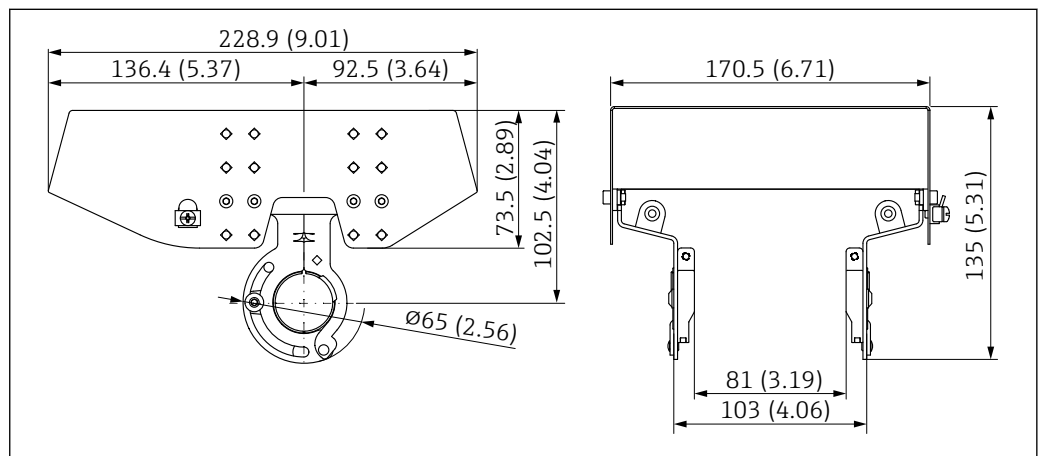
64 Dimensions of weather protection cover, 316 L, XW112. Unit of measurement mm (in)
