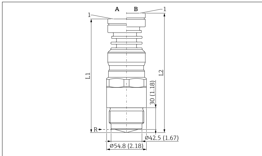
57 Dimensions; integrated antenna, PEEK, 40 mm (1.5 in); process connection, thread 1-½". Unit of measurement mm (in)
