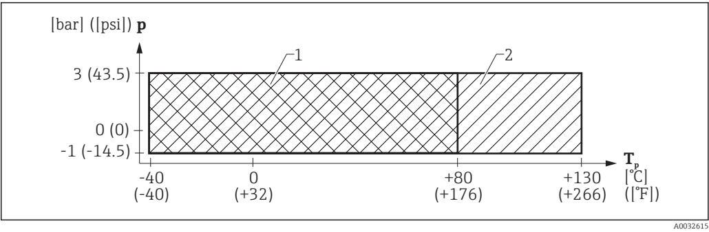
16 FMR60: Permitted range for process temperature and process pressure
