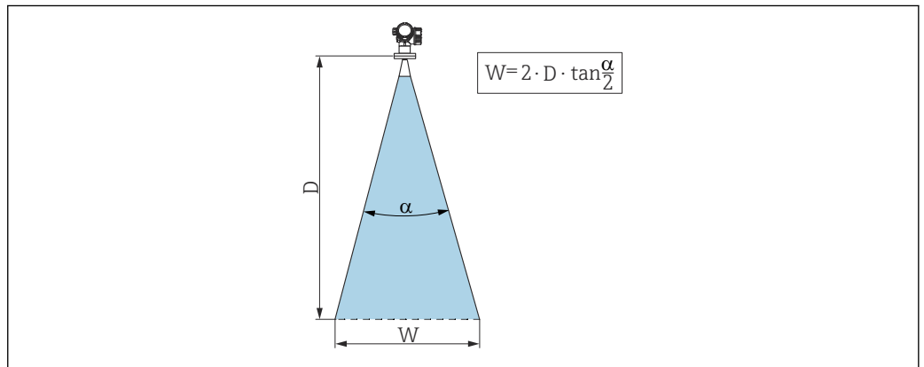
18 Relationship between beam angle \alpha , distance D and beam width W
