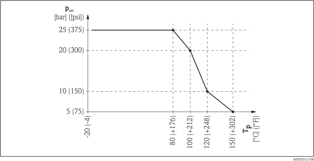
23 FMR54 with planar antenna: Permitted range for process temperature and process pressure
