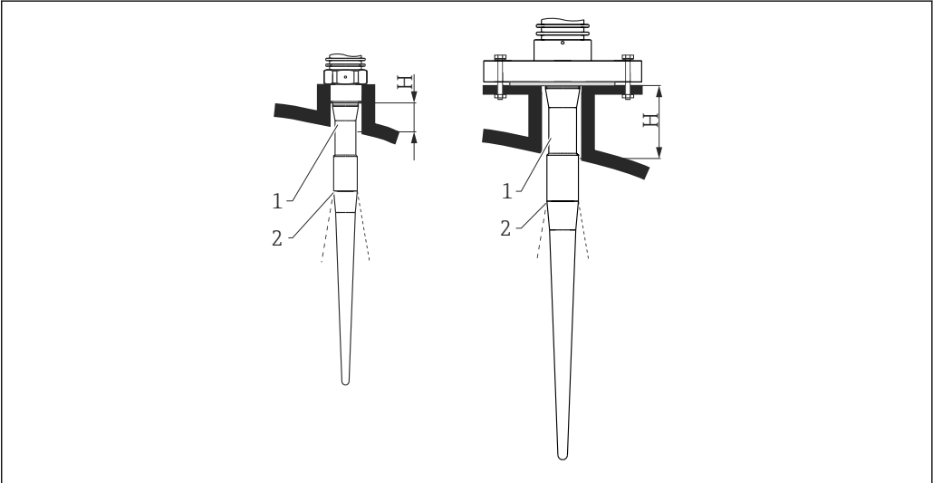
19 Nozzle height for rod antenna (FMR53)
