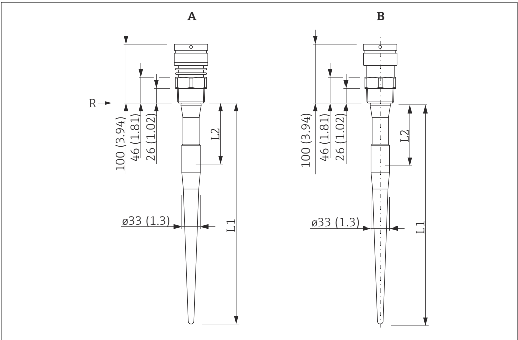
28 Dimensions of device with thread. Unit of measurement mm (in)
