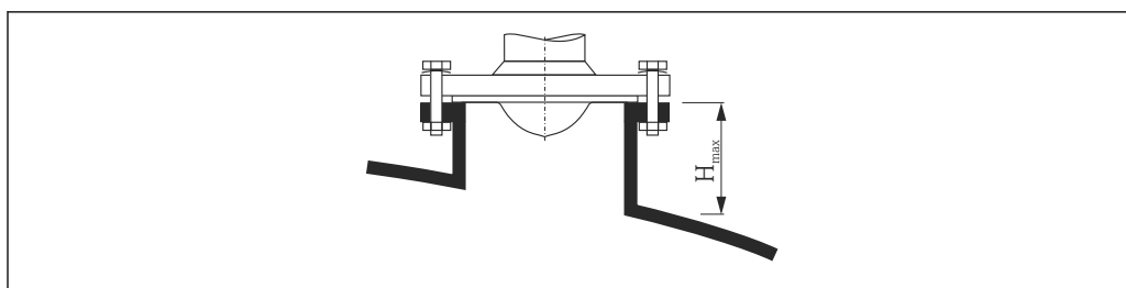
22 Nozzle height for horn antenna, flush mount (FMR52)
