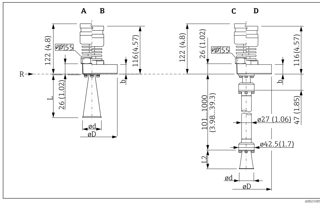
33 Dimensions of antenna, version T < 250\text{ °C} (482 °F). Unit of measurement mm (in)
