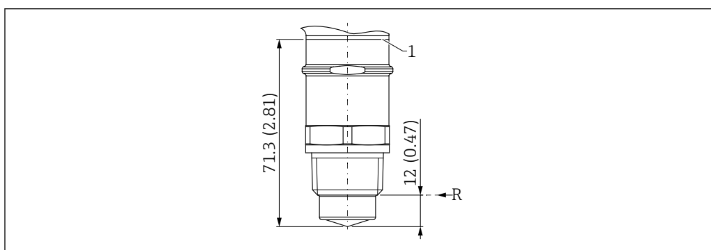
12 Dimensions; process connection MNPT \frac{3}{4} , 80 GHz; PEEK
