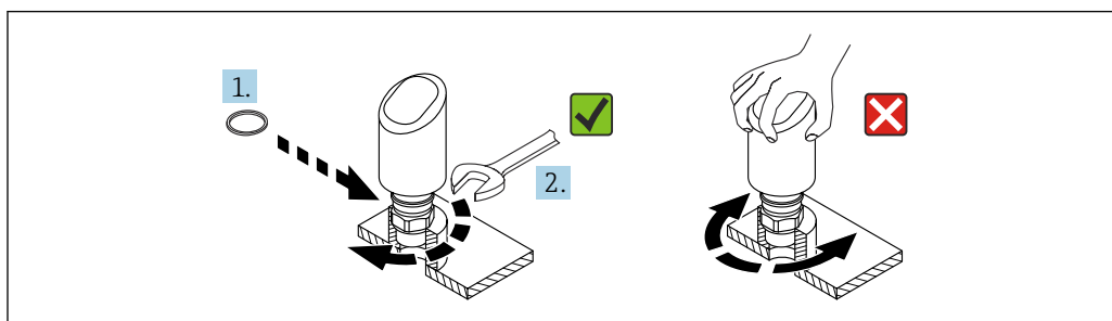
6 Screwing in the device
