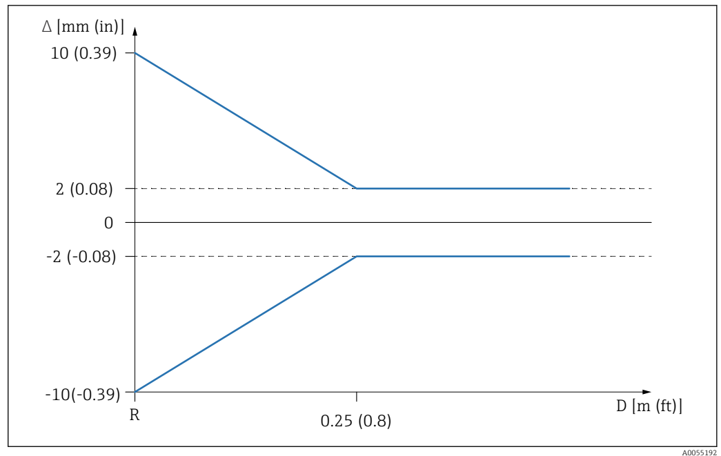
9 Maximum measurement error in near-range applications
