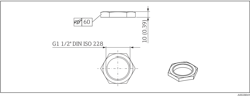
31 Dimensions of securing nut. Unit of measurement mm (in)
