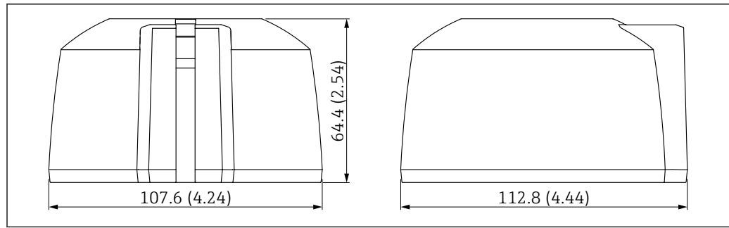
20 Dimensions for weather protective cover G1/NPT1, cable entry from above. Unit of measurement mm (in)
