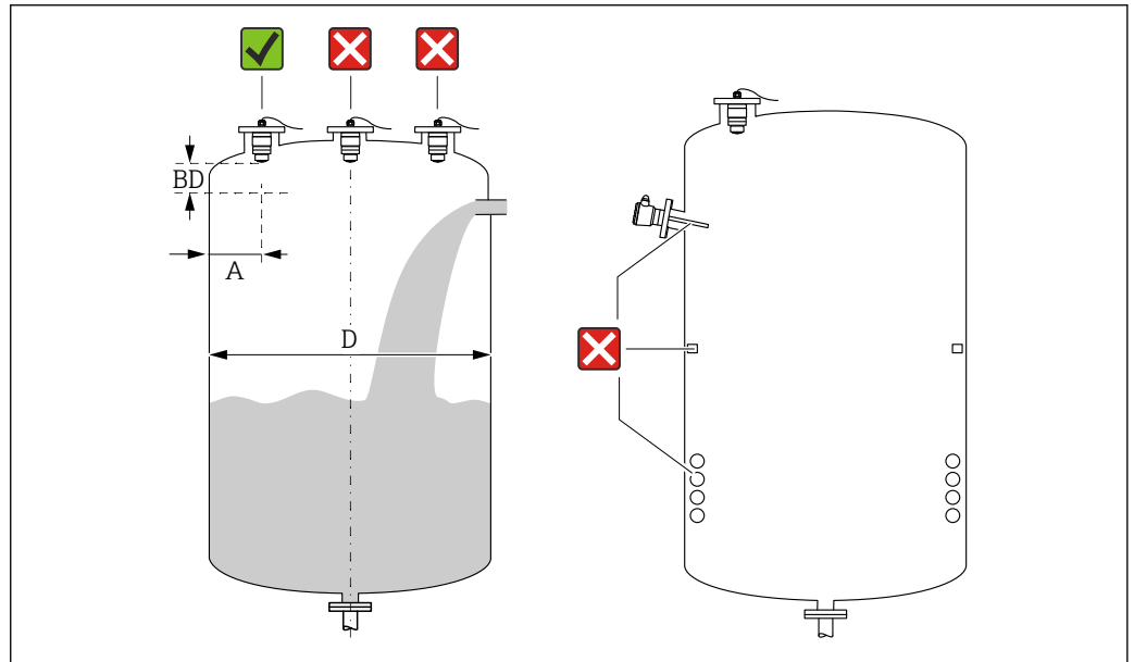
8 Installation position on a vessel
