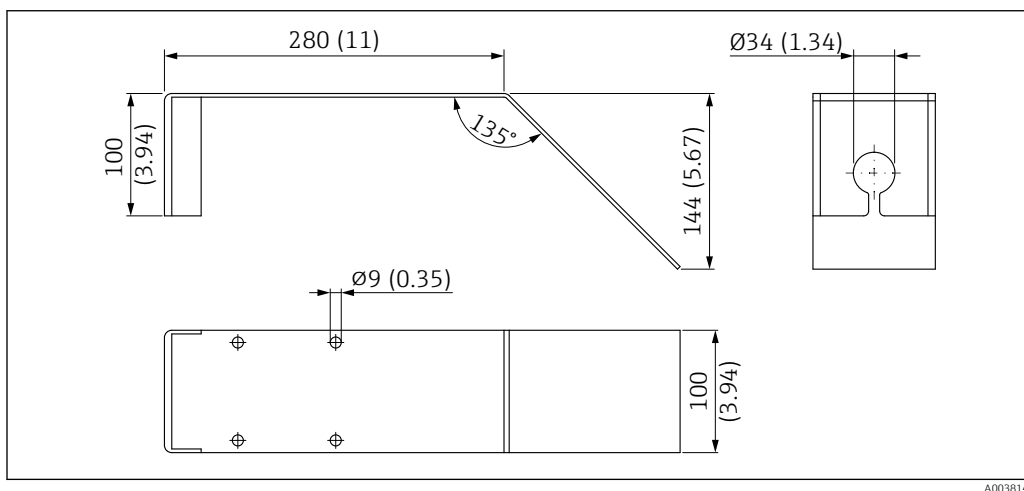
41 Dimensions of horizontal mounting bracket for sewer shafts. Unit of measurement mm (in)
