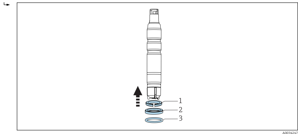
5 Slide clamping ring (1), thrust collar (2) and O-ring (3) upwards from the membrane cap to the sensor shaft and into the lower groove.
