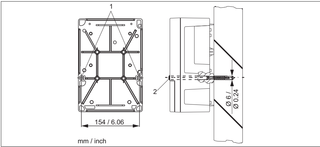
Wall mounting of the field instrument
