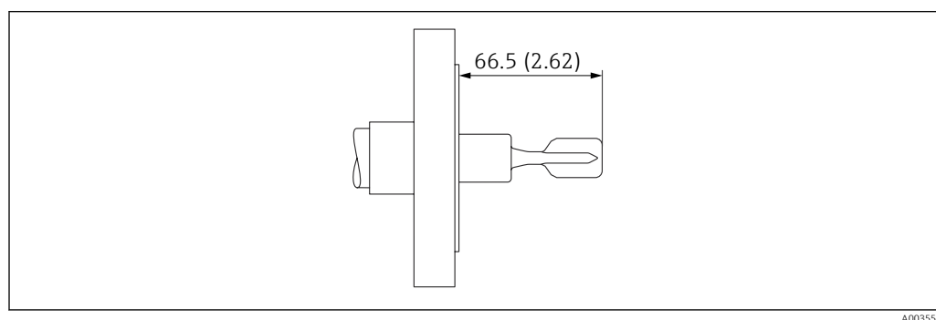
47 Example with flange. Unit of measurement mm (in)
