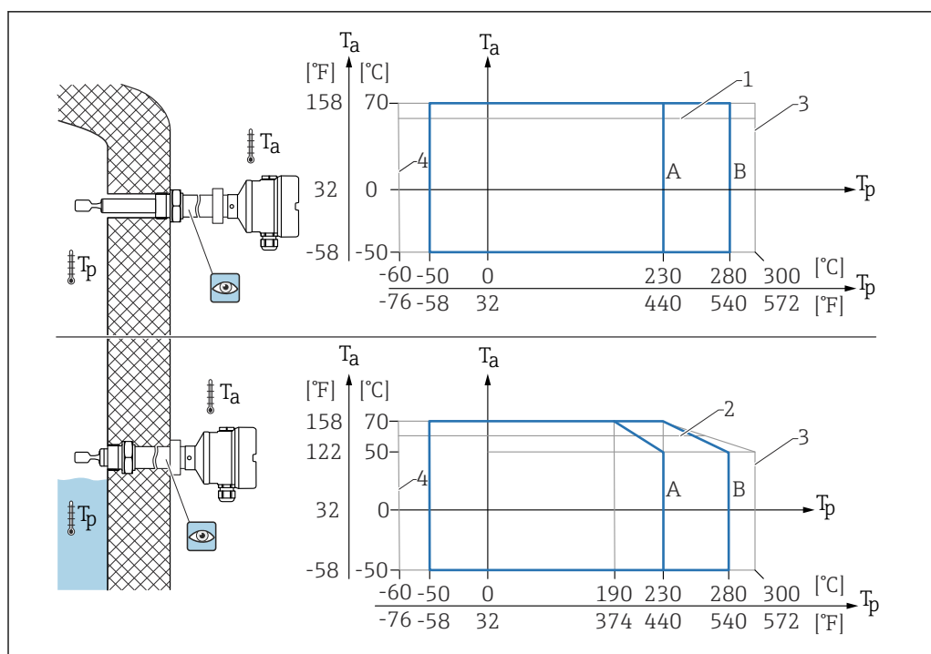
28 Permitted ambient temperature T_a at the housing as a function of the process temperature T_p in the vessel
