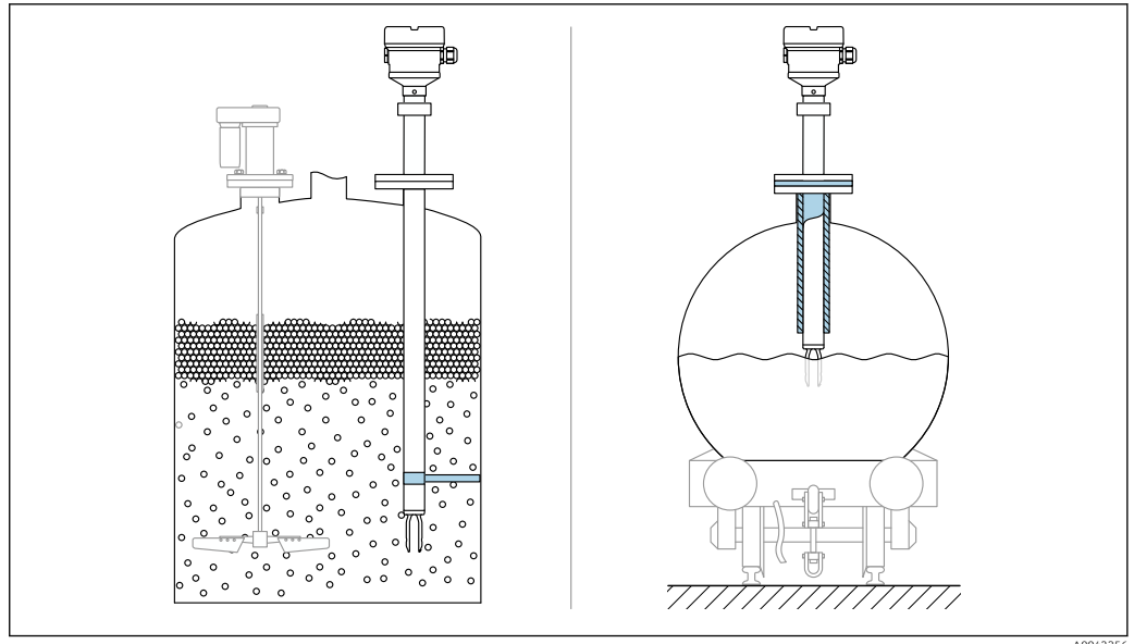
27 Examples of support in the event of dynamic load
