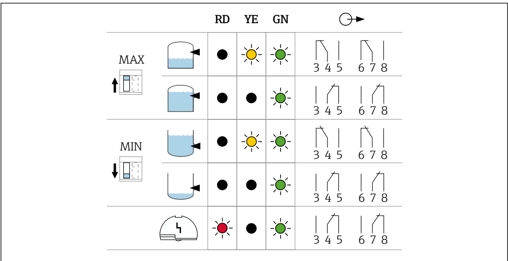
8 Behavior of switch output and signaling, electronic insert FEL64 MAX DIP switch for setting MAX safety mode MIN DIP switch for setting MIN safety mode RD LED red for alarm YE LED yellow, switch status GN LED green, operational status, device on
