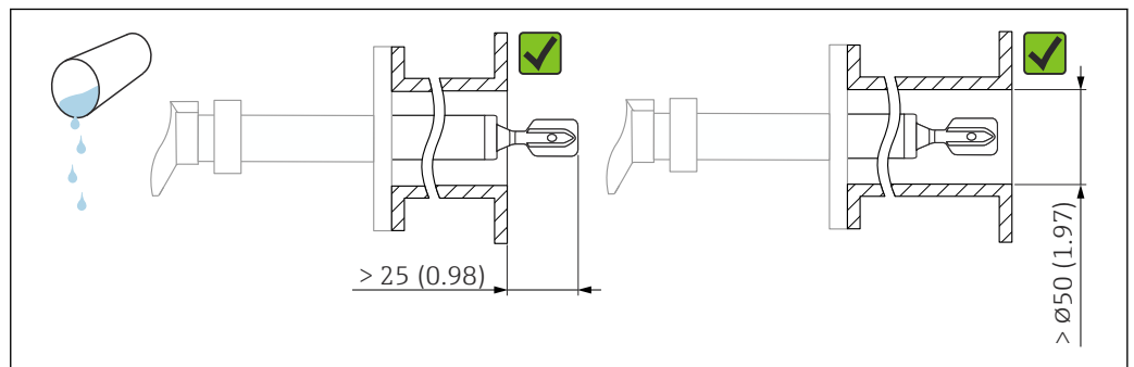
19 Installation example for low-viscosity liquids. Unit of measurement mm (in)
