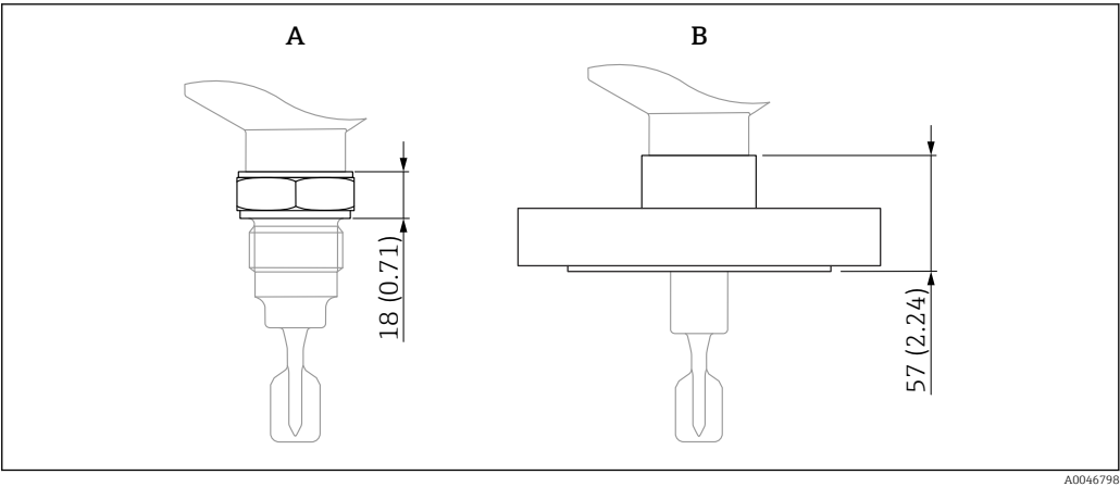
40 Maximum height specification for the process connections
