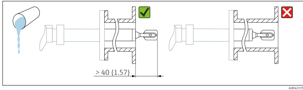
20 Installation example for a highly viscous liquid. Unit of measurement mm (in)
