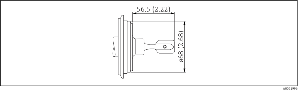
29 Varivent N pipe DN65-162 PN25. Unit of measurement mm (in)
