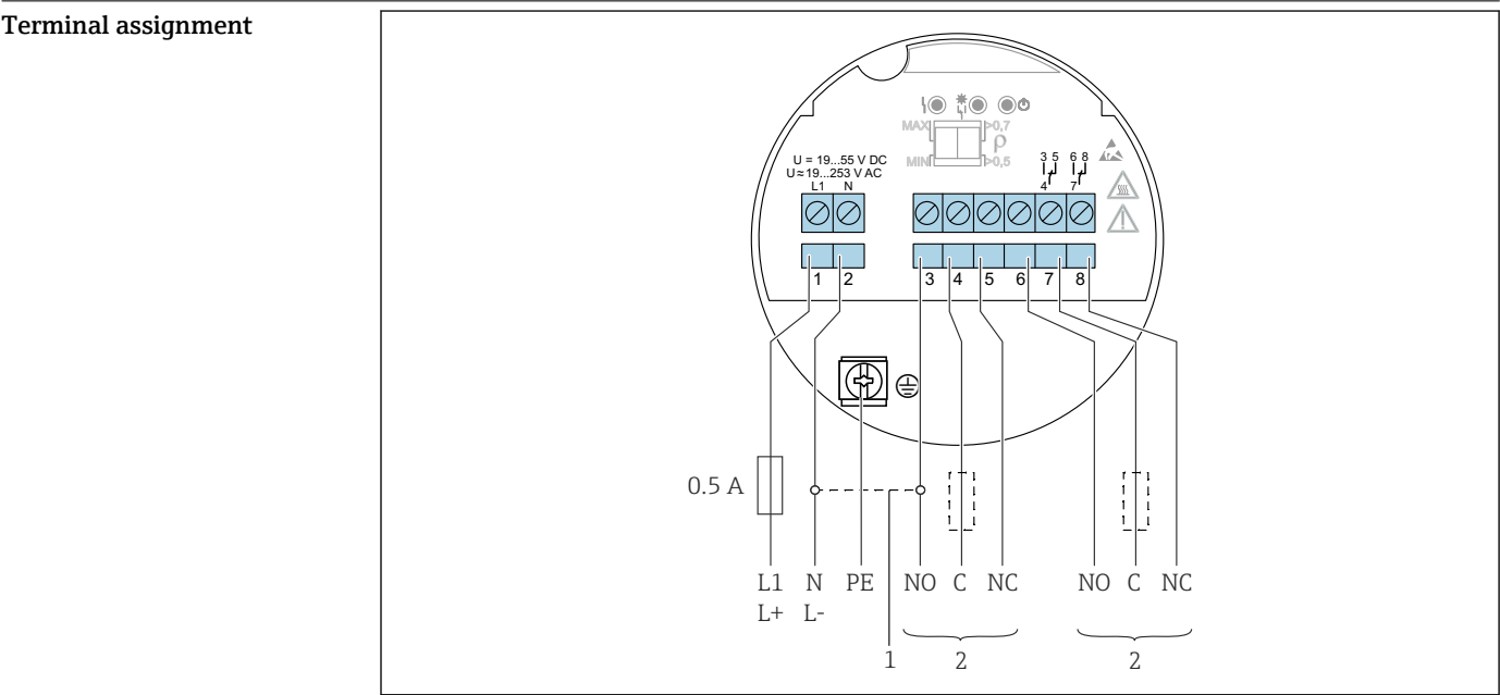
4 Universal current connection with relay output, electronic insert FEL44 1 When bridged, the relay output works with NPN logic 2 Connectable load
