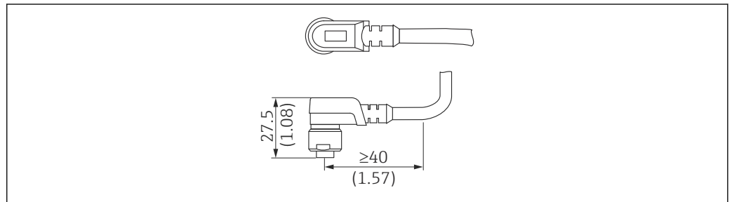
45 Plug-in jack M12 IP67. Unit of measurement mm (in)
