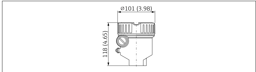
25 Single compartment; aluminum, coated; suitable for Ex d/XP area
