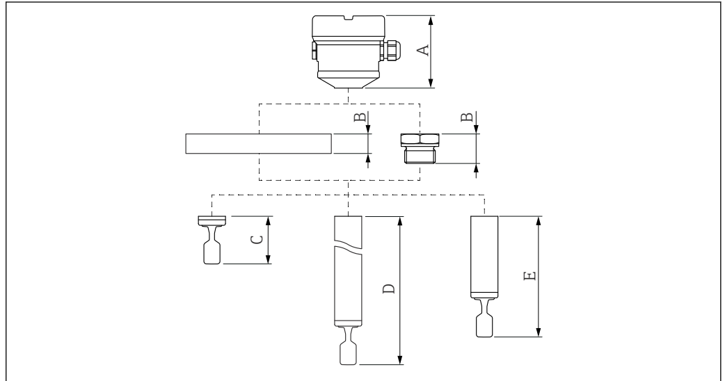
22 Components to determine the device height
