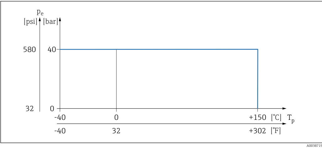
21 Process temperature FTL41
