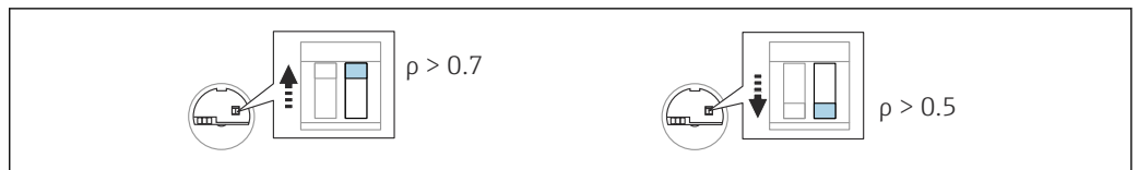
42 Switch position on the electronic insert for density
