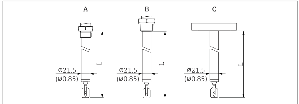
27 Probe designs: pipe extension, short pipe, sensor length L
