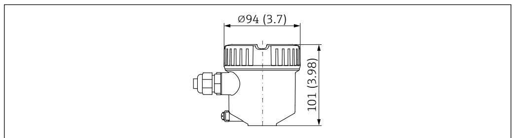
23 Single compartment; plastic housing
