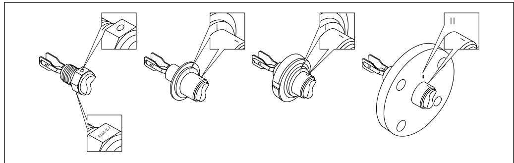
15 Markings to align the tuning fork
