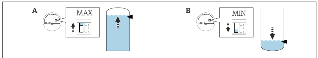
41 Switch position on the electronic insert for MAX/MIN safety mode
