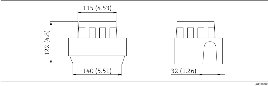
43 Protective cover for single compartment housing, aluminum or 316L. Unit of measurement mm (in)
