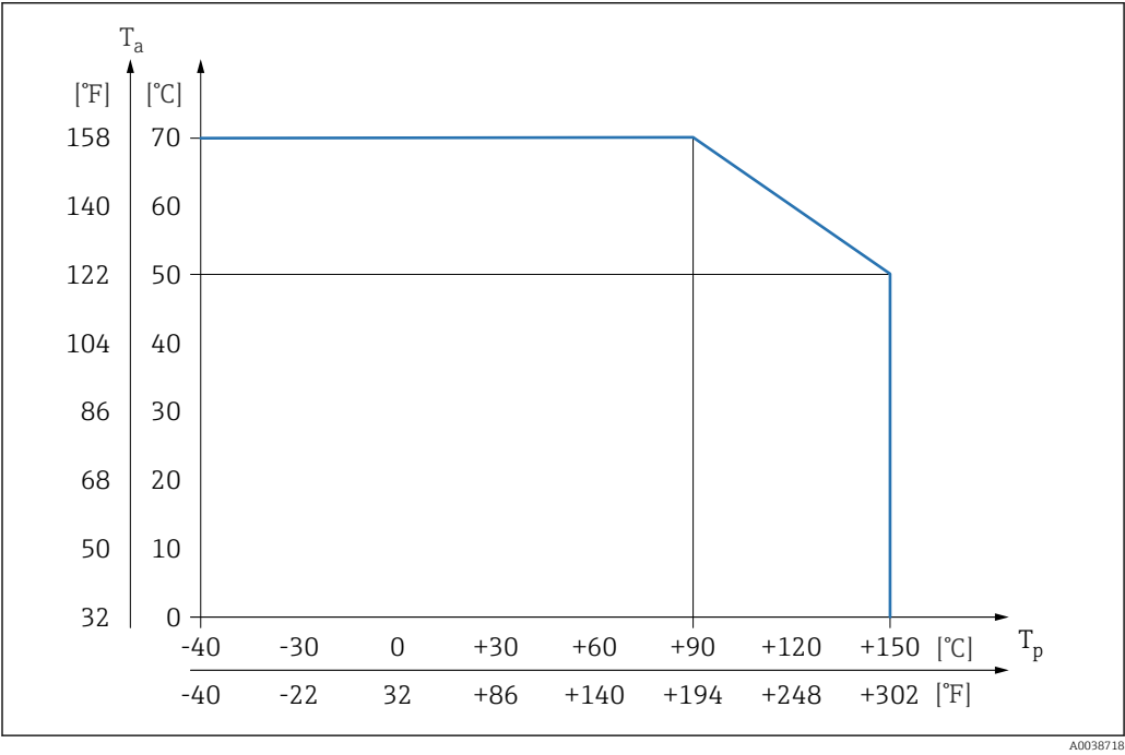
20 At process temperature and FEL44 T_p > 90\text{ °C} max. load current 4 A
