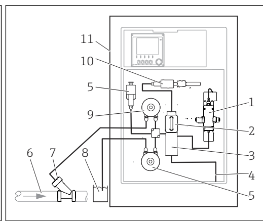
3 Measuring system with Liquiline System CA80TP and Y strainer
