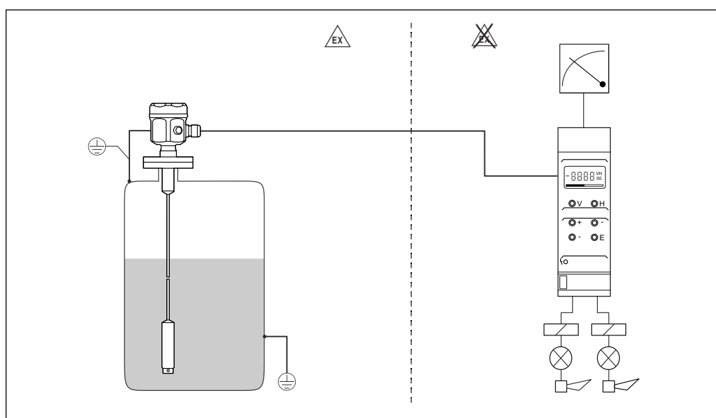
1 Level measurement
