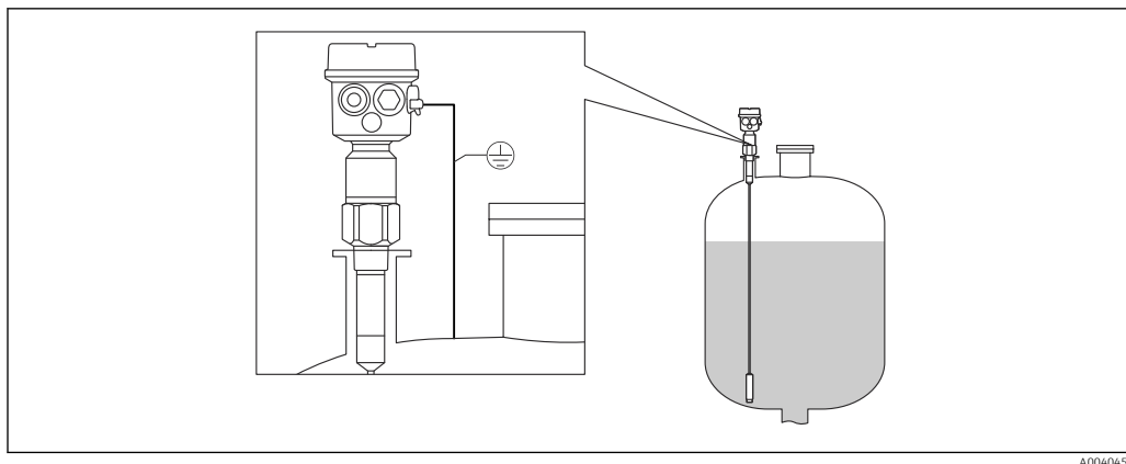
5 A probe with fully insulated inactive length for mounting nozzles
