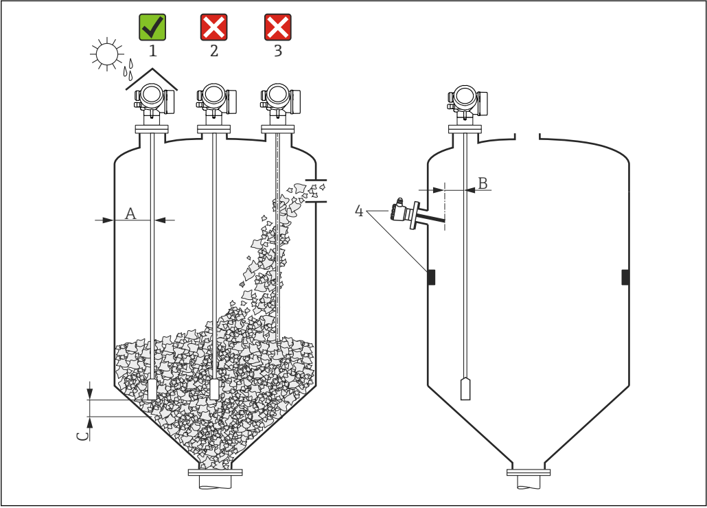
25 Installation positions
