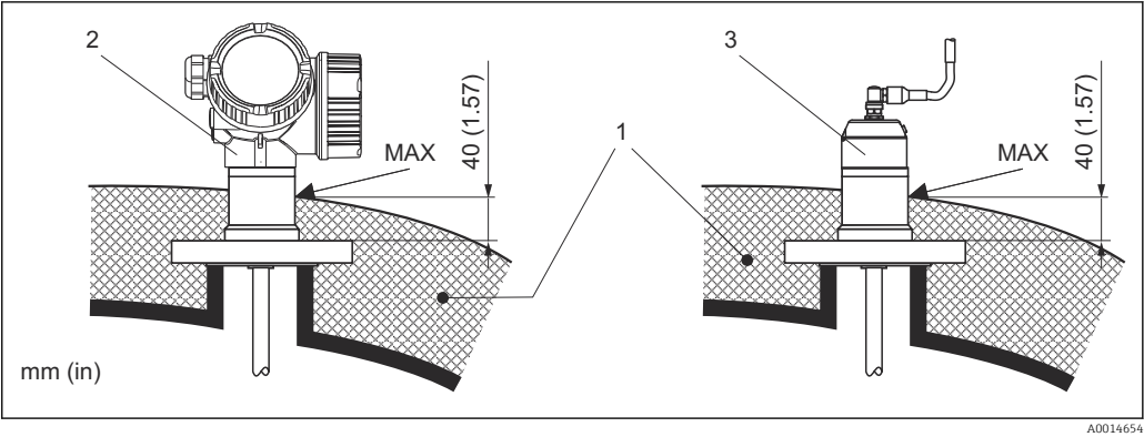
32 Process connection with flange - FMP57
