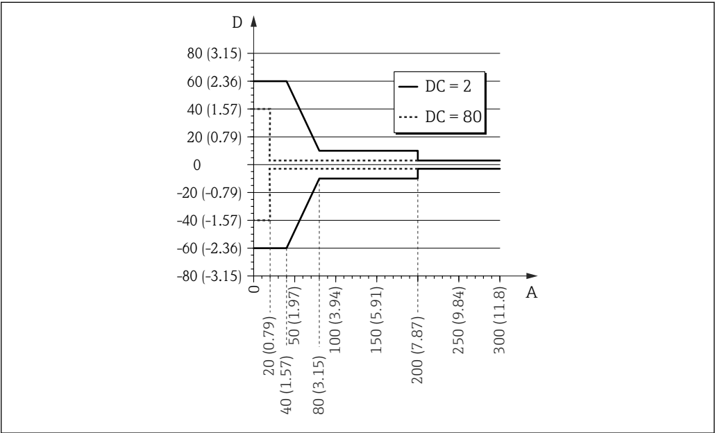
22 Measurement error at the probe end for rod and coaxial probes A Distance from the probe end [mm(in)] D Measurement error: Sum of non-linearity, non-repeatability and hysteresis DC Dielectric constant ( \epsilon_r )
