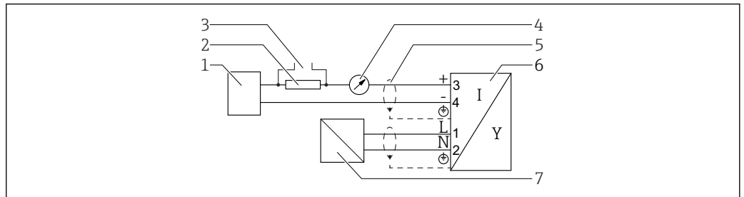
18 Function diagram 4-wire: 4 to 20 mA HART (90 to 253 V AC )
