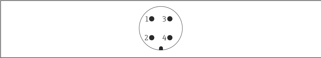
23 Pin assignment of 7/8" plug
