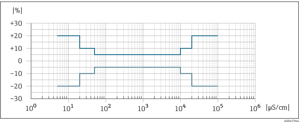
26 Measured error (optional: order code for "Calibrated conductivity measurement", option CW)
