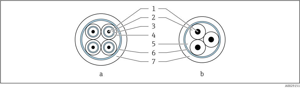
22 Cable cross-section
