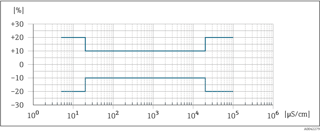
25 Measured error (standard)
