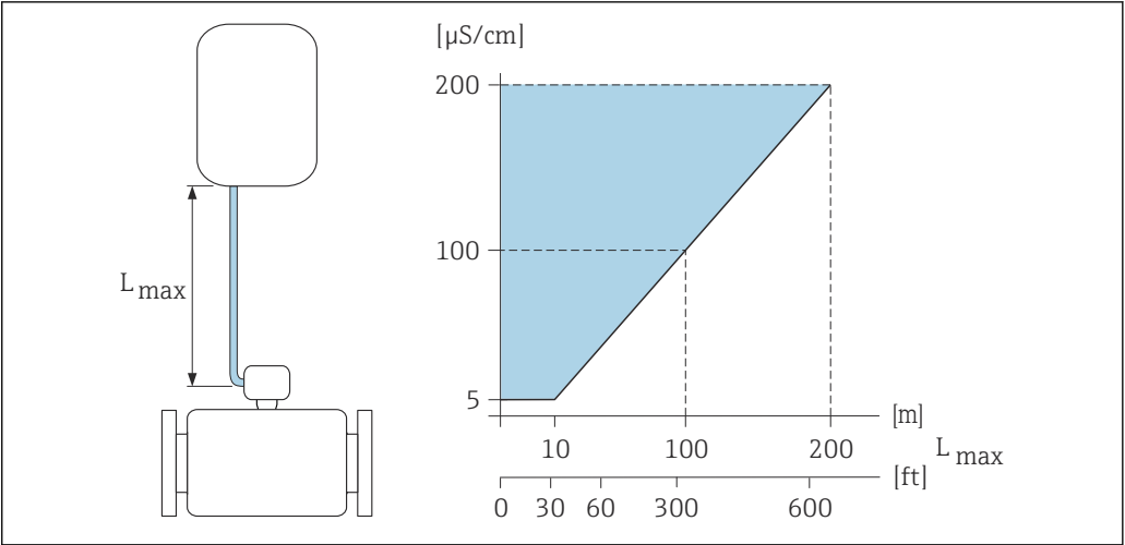
27 Permitted length of connecting cable Colored area = permitted range L_{max} = length of connecting cable in [m] ([ft]) \mu S/cm = medium conductivity
