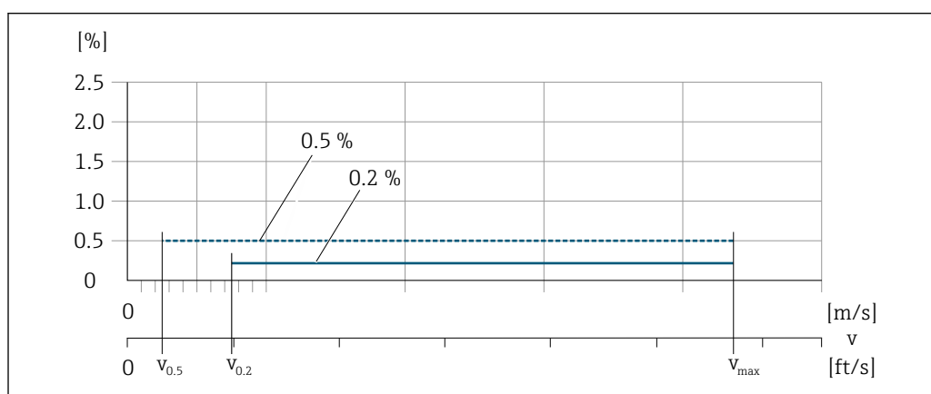
24 Flat Spec in % o.r.
