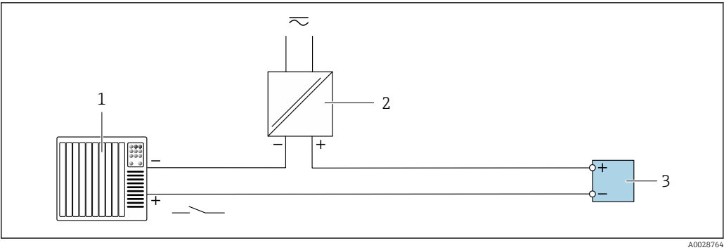
12 Connection example for status input
