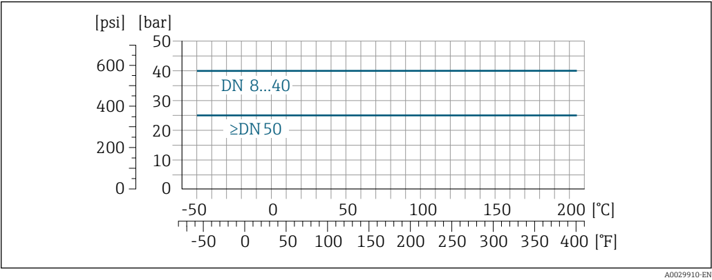
36 With connection material 1.4435 (316L)
