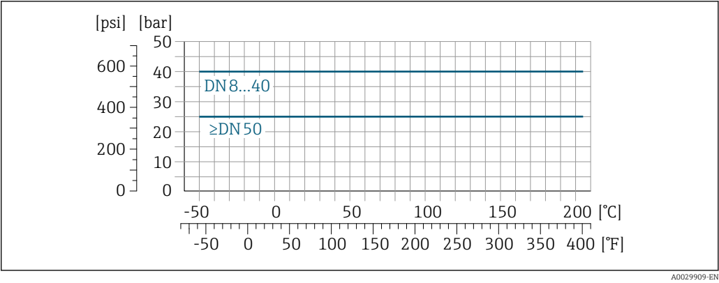
35 With flange material 1.4435 (316L)
