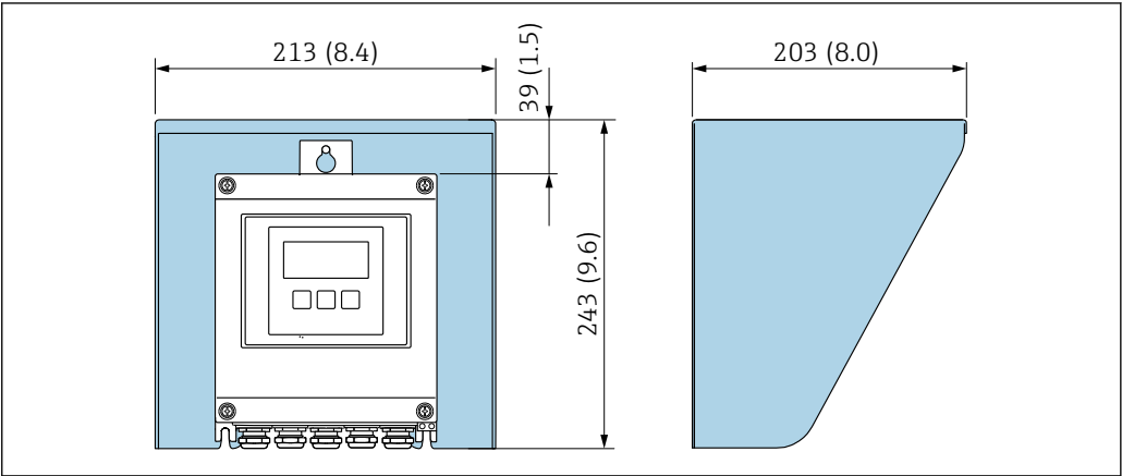
21 Weather protection cover for Proline 500 – digital
