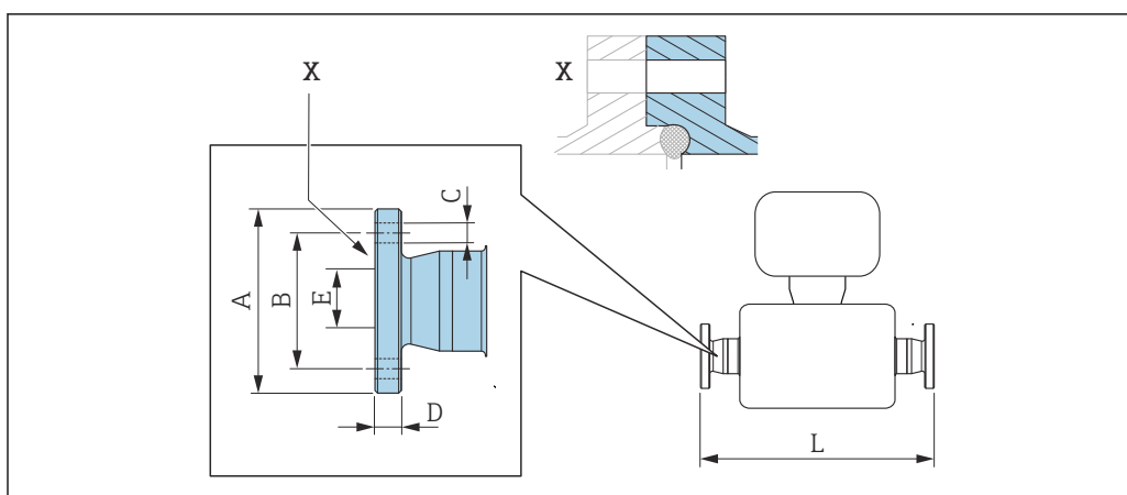
59 Detail X: Asymmetrical process connection; the part shown in blue is provided by the supplier.
