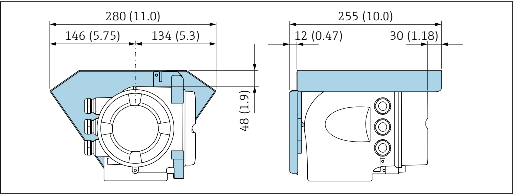
65 Weather protection cover for Proline 500; engineering unit mm (in)
