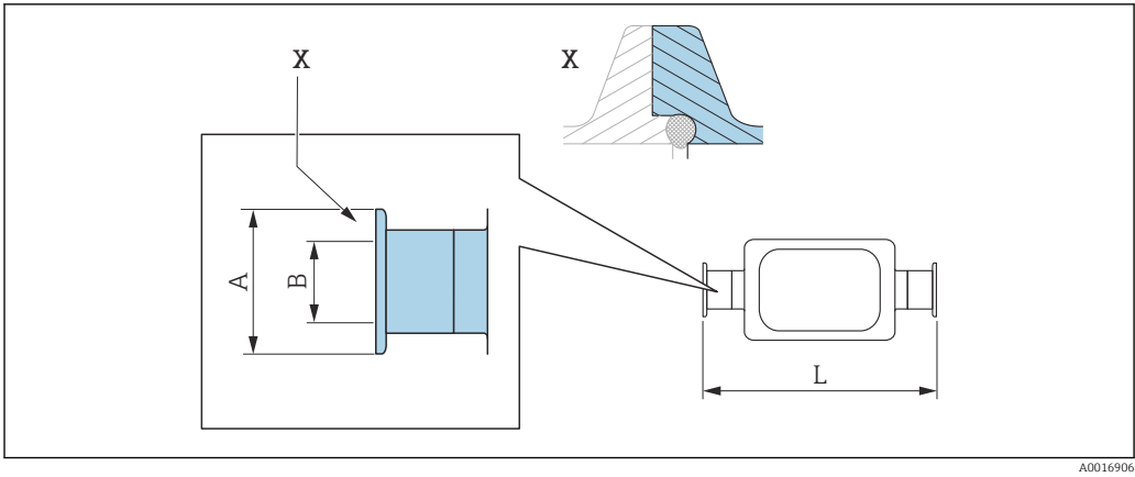
51 Detail X: Asymmetrical process connection; the part shown in blue is provided by the supplier.
