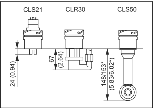
9 Length below the sensor holder
