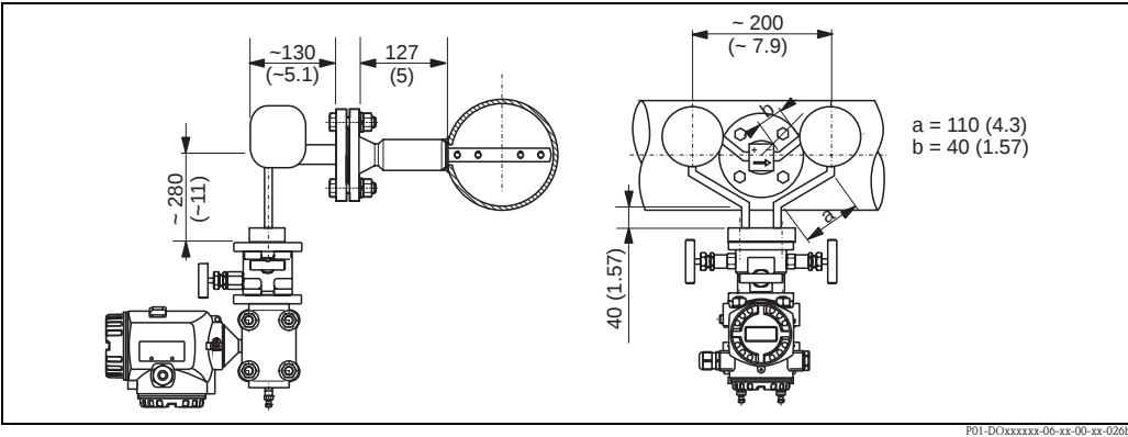
For steam in horizontal pipes; mounting right Dimensions in mm (inch)
