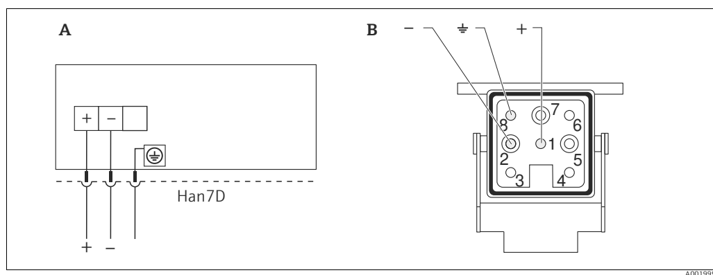
A Electrical connection for devices with Harting plug Han7D B View of the plug-in connection at the device
