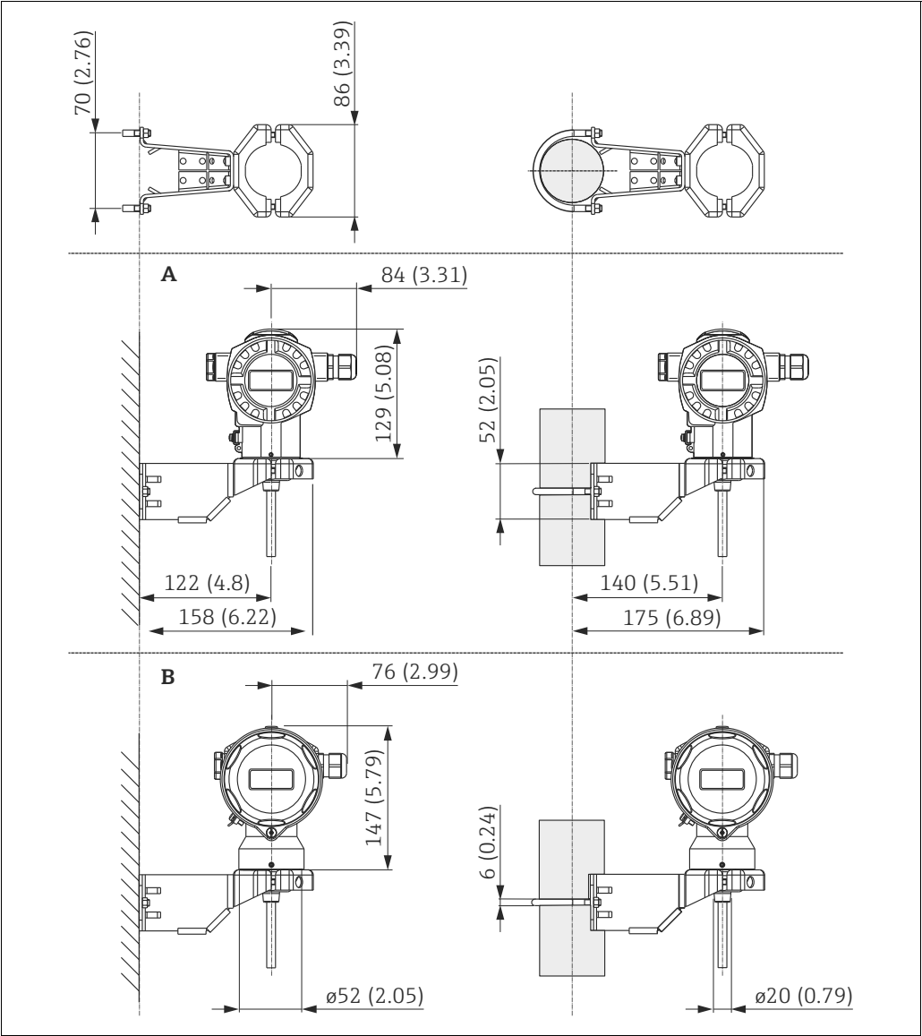
Measuring unit mm (in)
