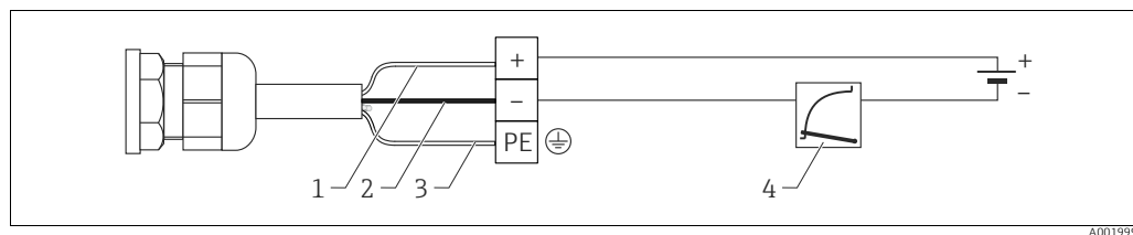
1 rd = red 2 bk = black 3 gnye = green 4 20 mA
