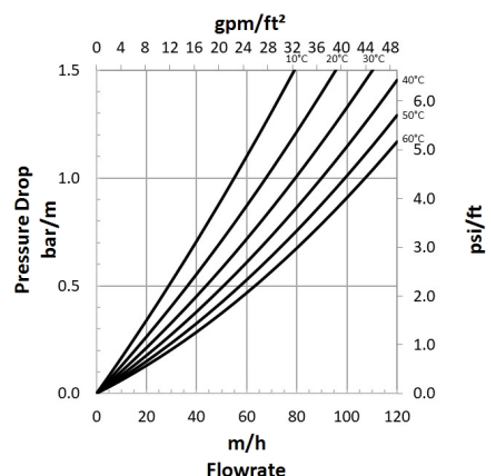
Figure 2: Pressure Drop
