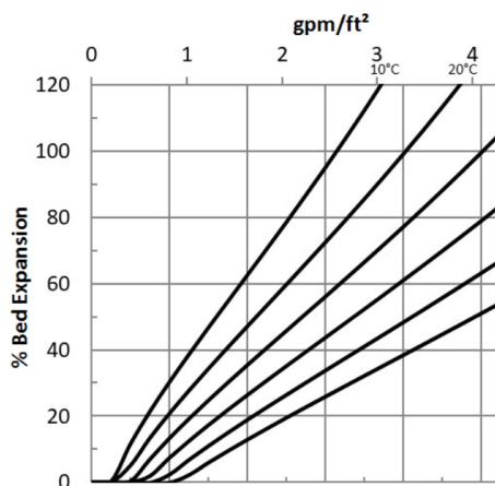
Figure 1: Backwash Expansion
